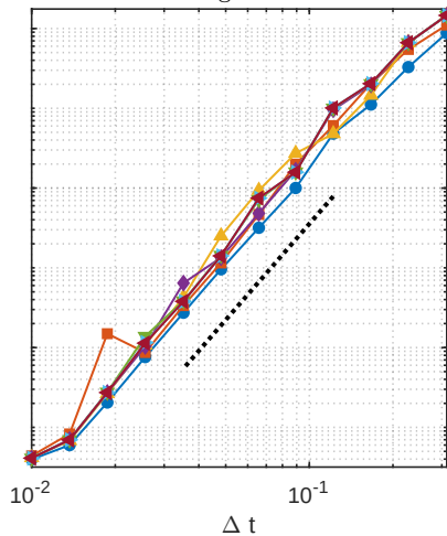
Convergence for v
