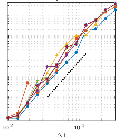
Convergence for w
