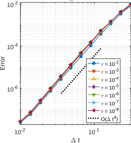
Convergence for u
