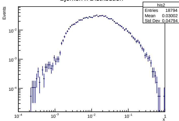
Bjorken x Distribution
