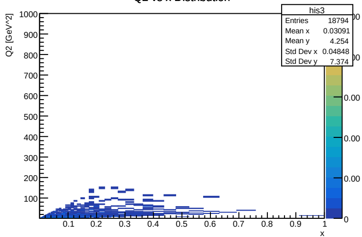
Q2 vs x Distribution
