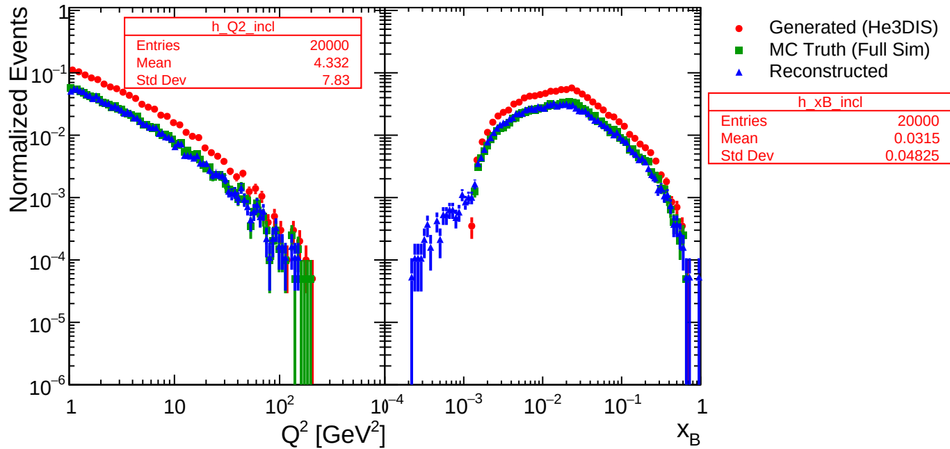
Q^2 Distribution
