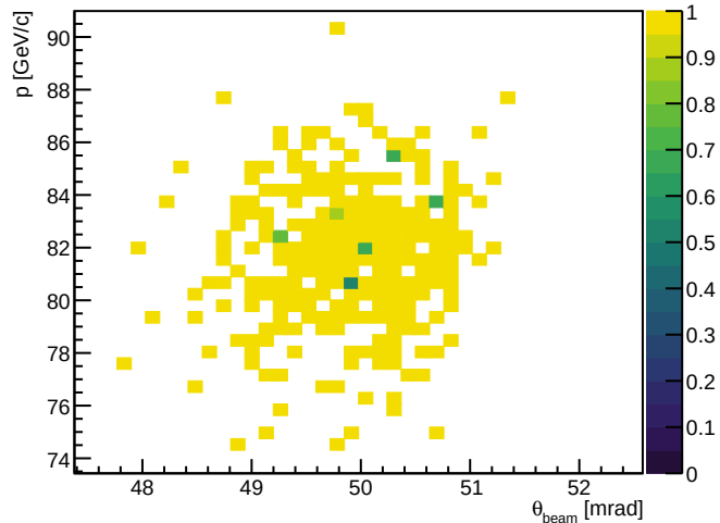
Deuteron RP acceptance, inclusive ( \geq 1 station)
