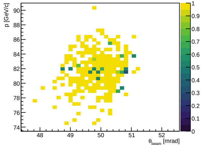
Deuteron RP acceptance, 2-of-2 coincidence
