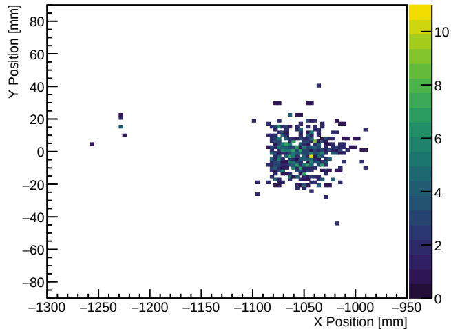
Deuterons: RP Station 1 ( z \approx 32.5 m)
