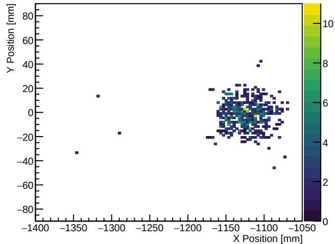
Deuterons: RP Station 2 ( z \approx 34.3 m)
