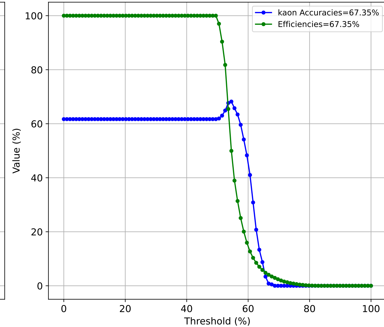
Accuracy and Efficiency Tradeoff (kaon)
