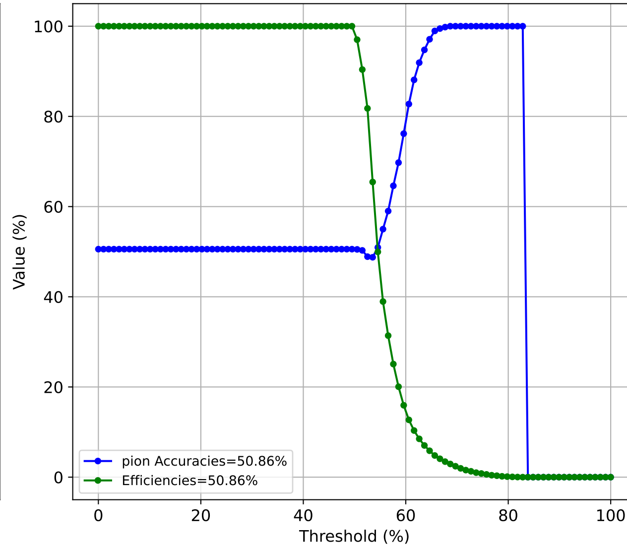
Accuracy and Efficiency Tradeoff (pion)
