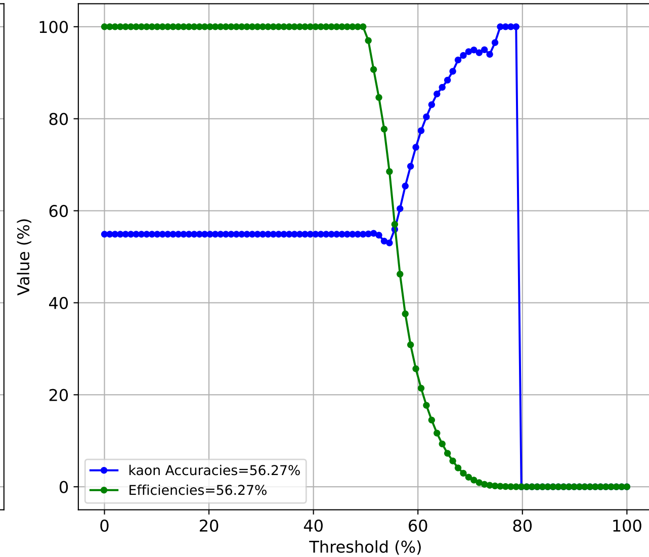
Accuracy and Efficiency Tradeoff (kaon)
