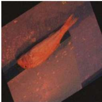
Augmented
