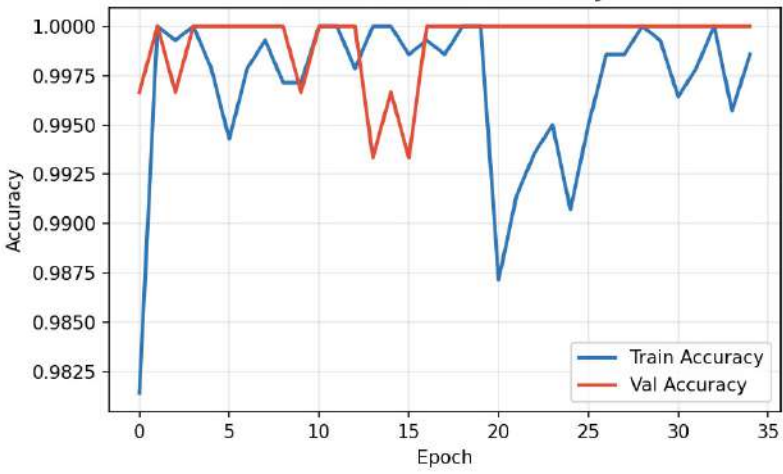
MOBILENETV2 — Accuracy
