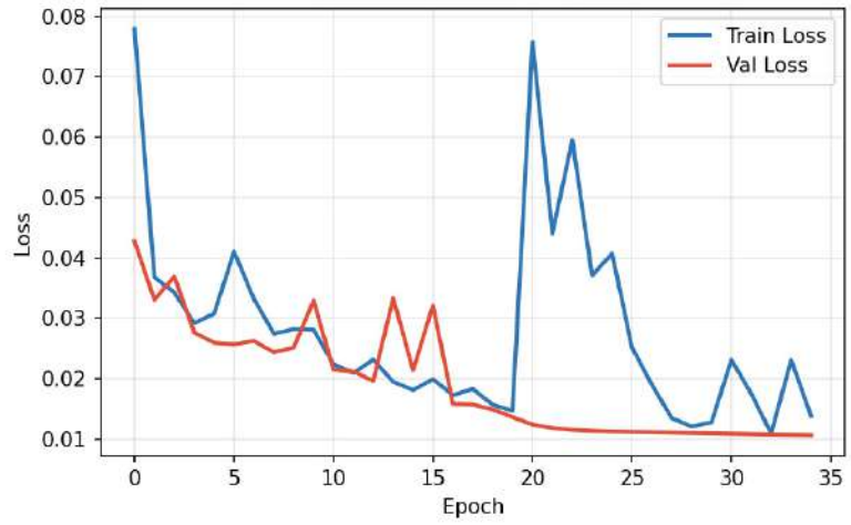
MOBILENETV2 — Loss
