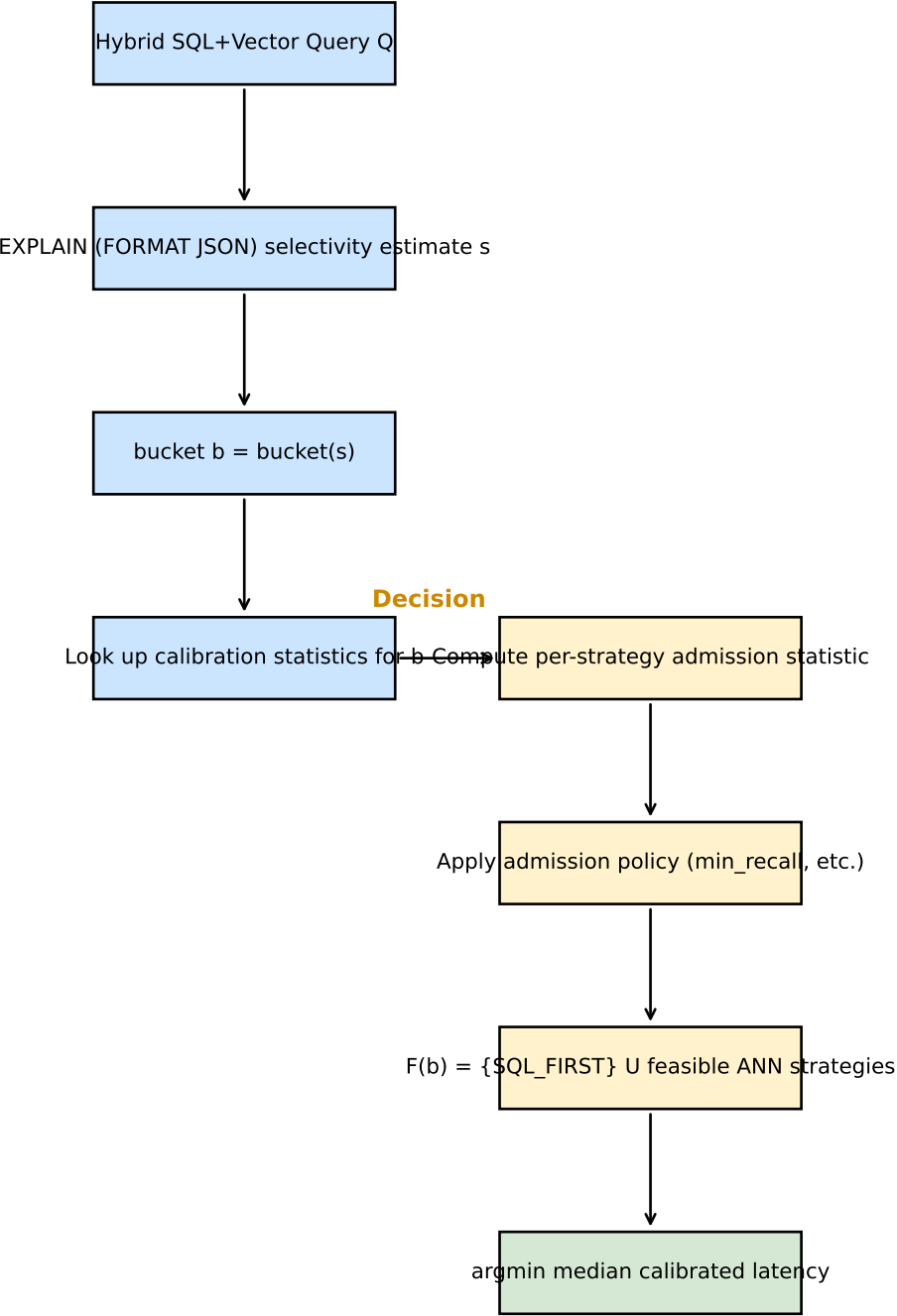
Figure 1: Adaptive Decision Flow
