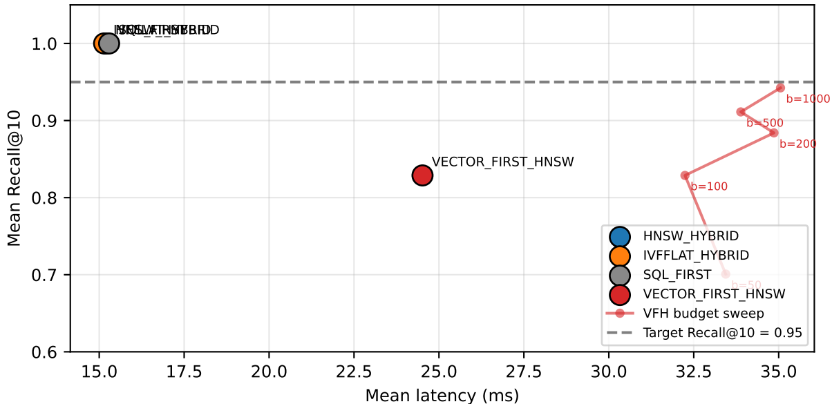
Latency-Recall Pareto frontier
