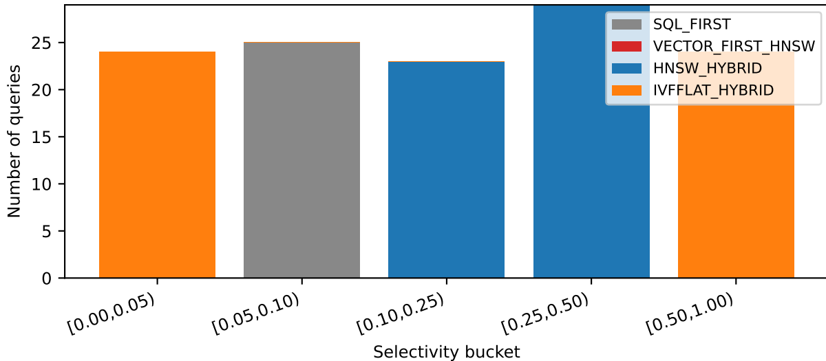
Adaptive selection by selectivity bucket
