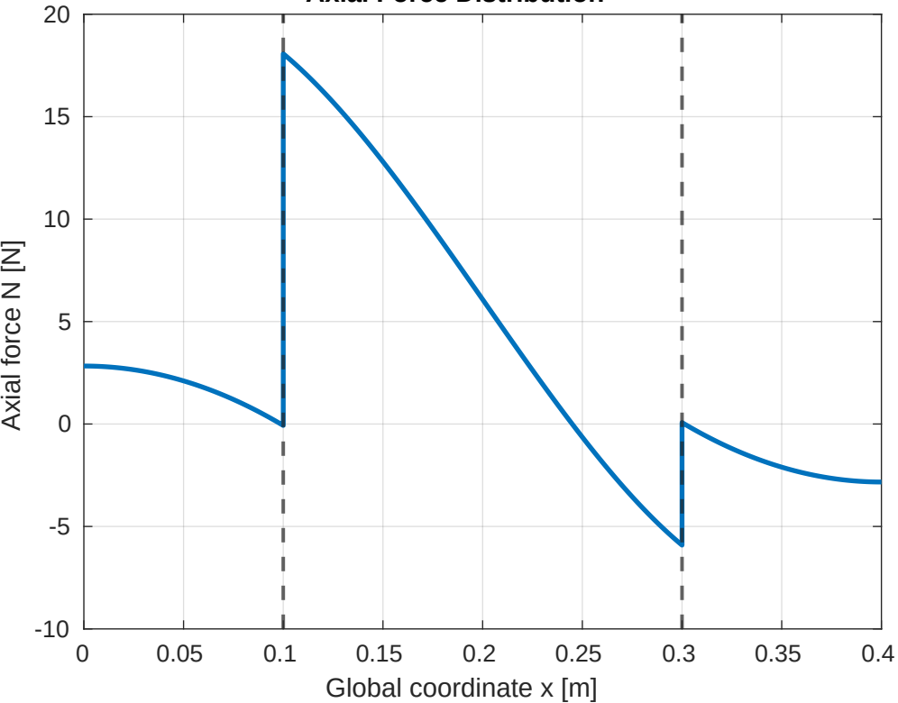
Axial Force Distribution
