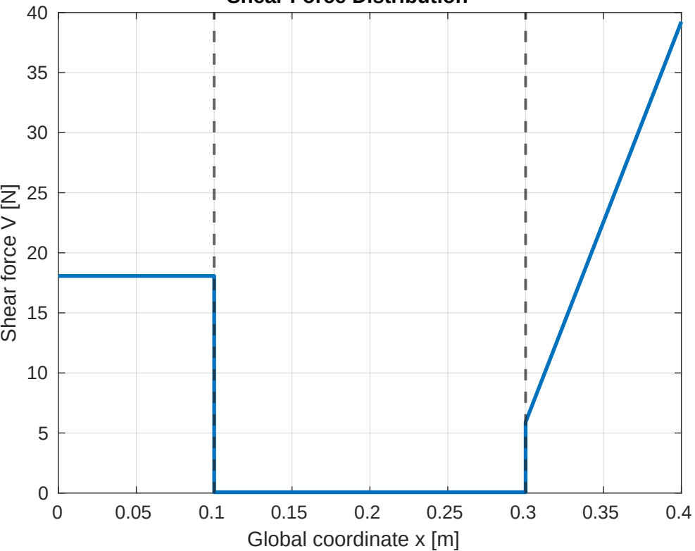
Shear Force Distribution
