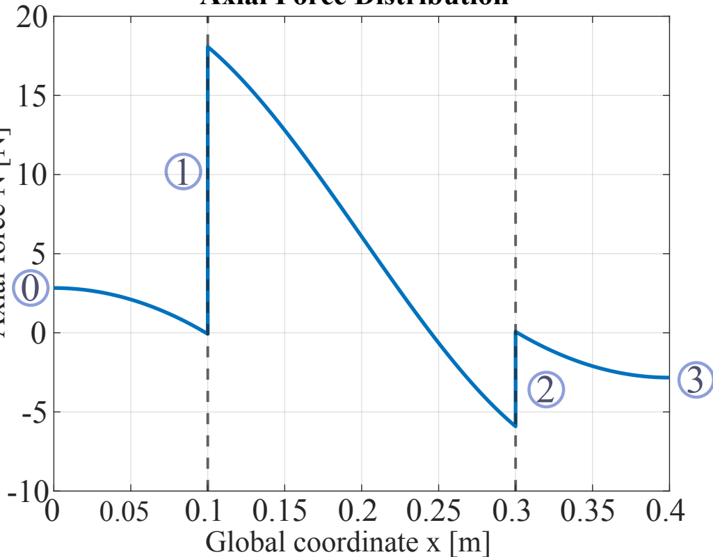
Axial Force Distribution
