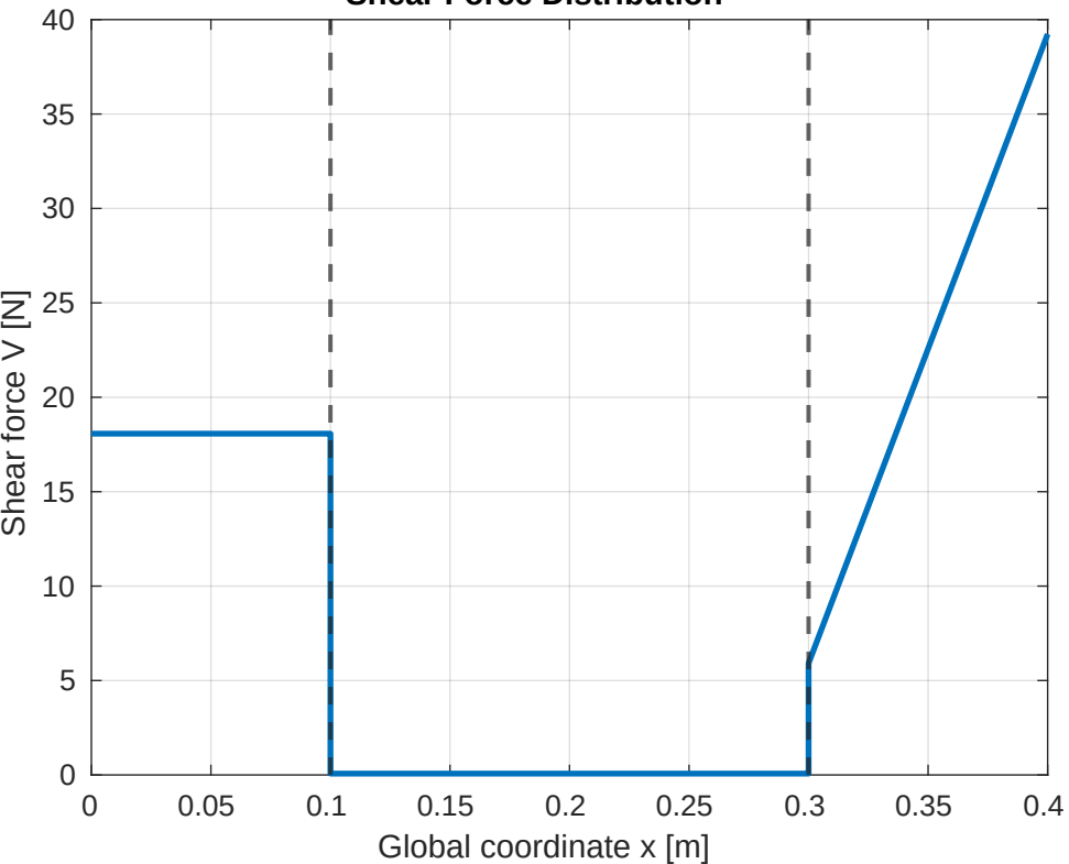
Shear Force Distribution
