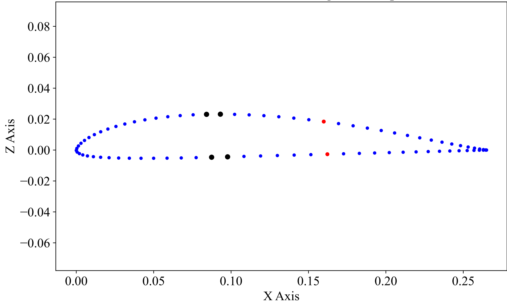
Airfoil Idealised Skin, Stringers and Spar
