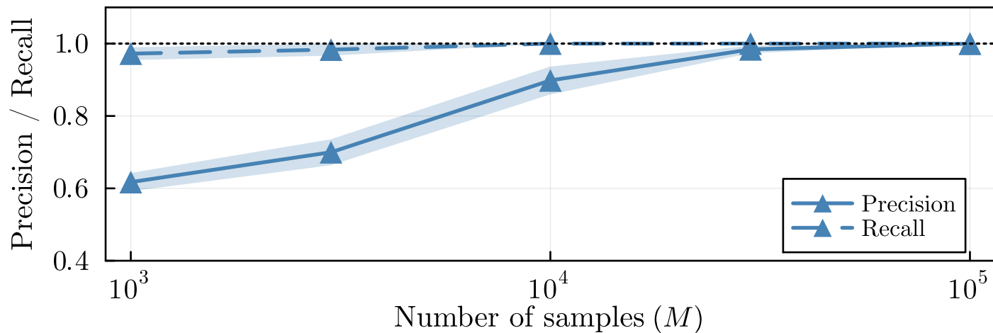
Structure learning, n = 24, \beta = 1.2
