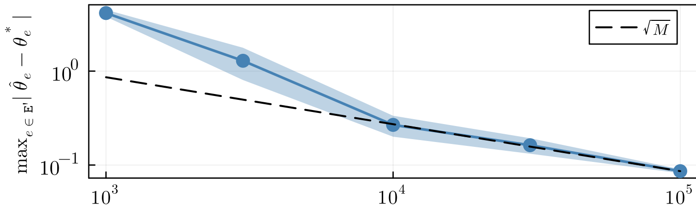
Structure learning, n = 24, \beta = 1.2
