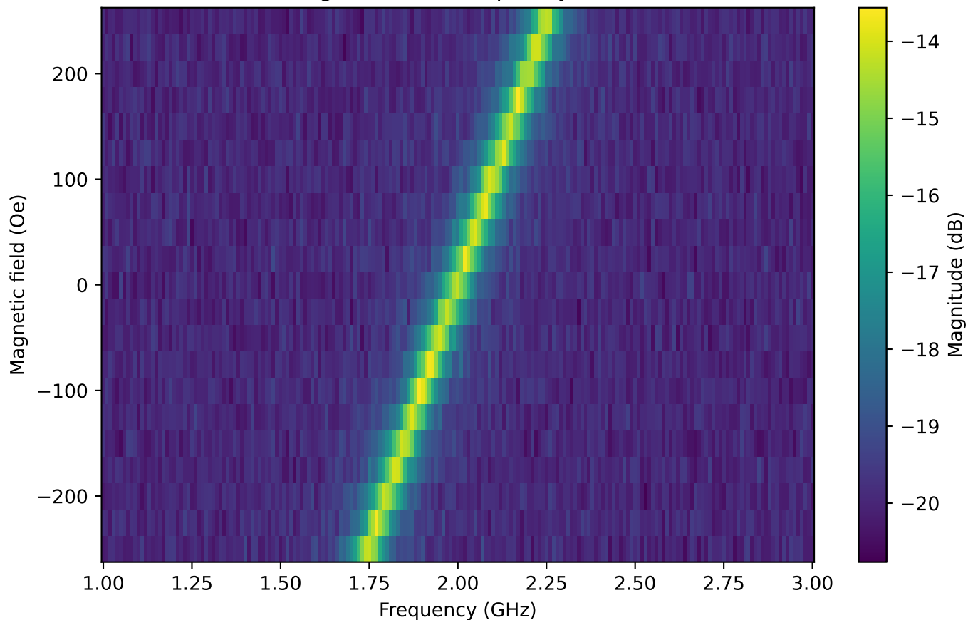
S11 Magnitude vs. Frequency and Field
