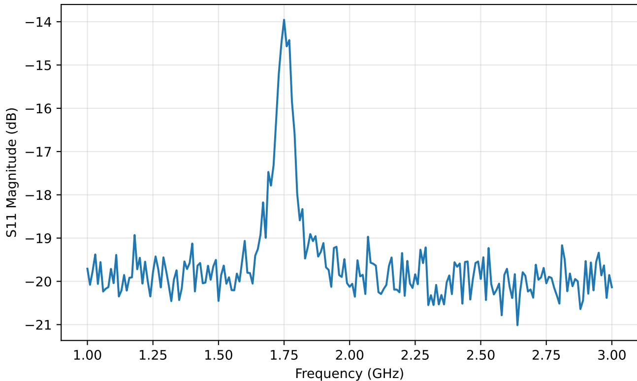
S11 at H=-250.0 Oe
