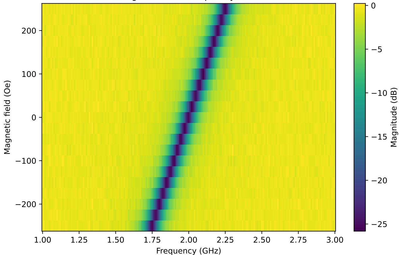
S21 Magnitude vs. Frequency and Field
