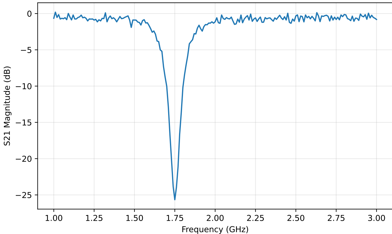
S21 at H=-250.0 Oe
