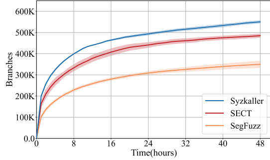
Figure 3: Code coverage achieved by Syzkaller, SegFuzz and SECT (N=10).
