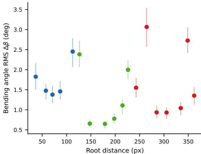
(b) Per-joint bending deviation with CI
