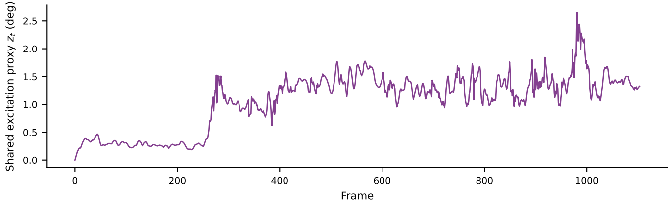
Estimated global airflow excitation over time
