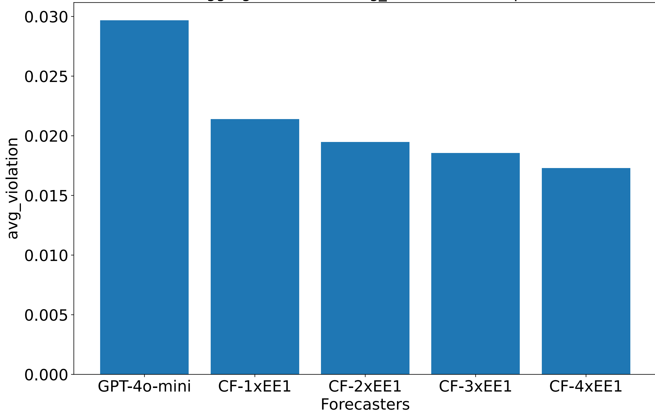
aggregated.default.avg_violation (newsapi)
