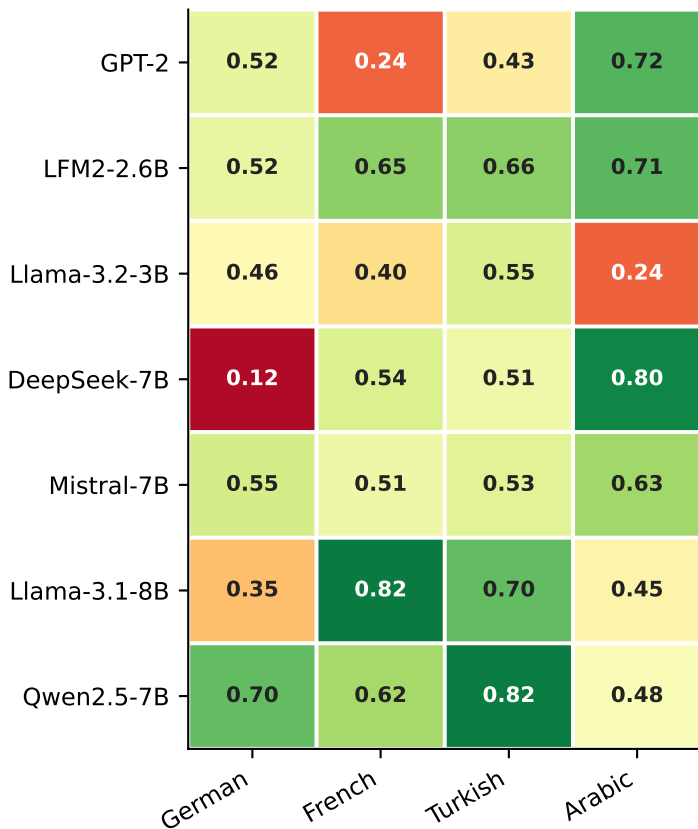
Attention Extractor
