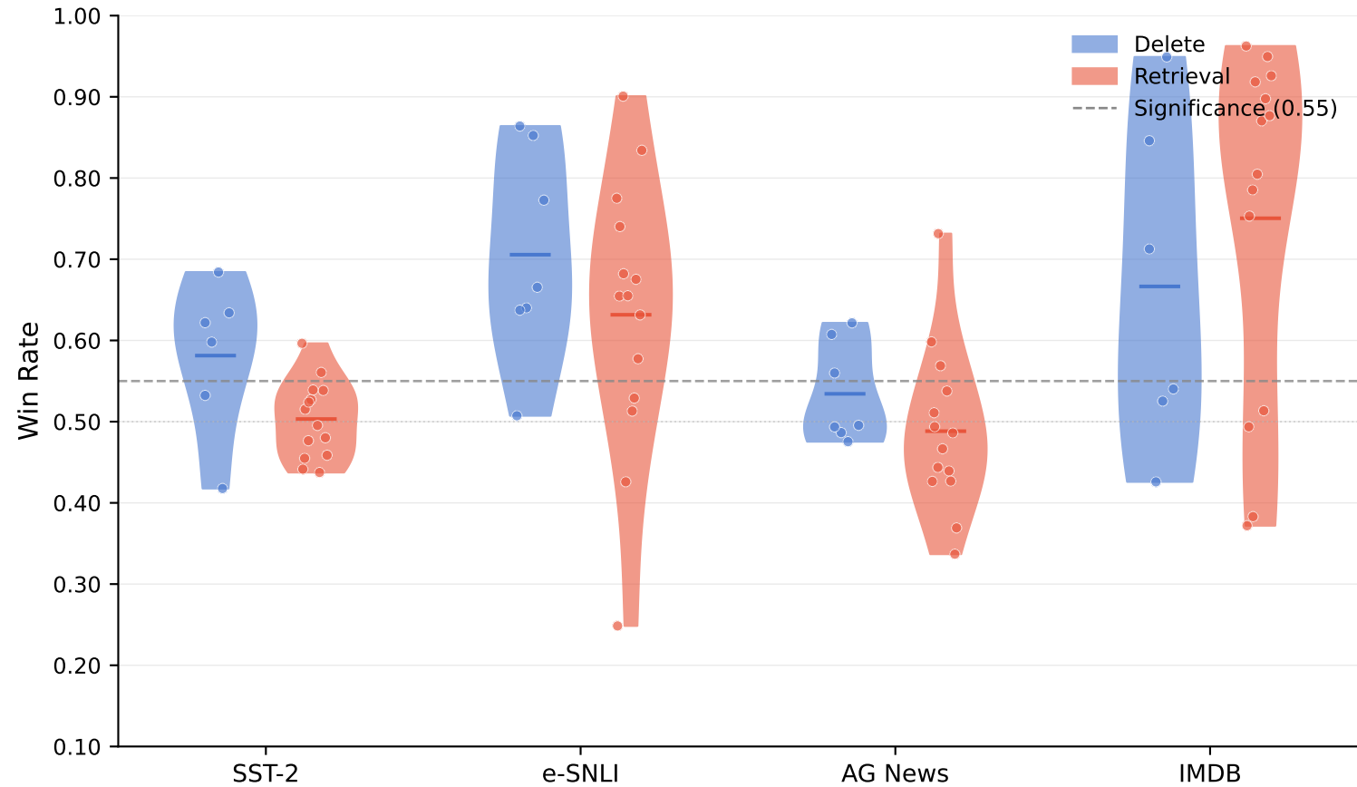
Distribution of Win Rates by Dataset and Operator
