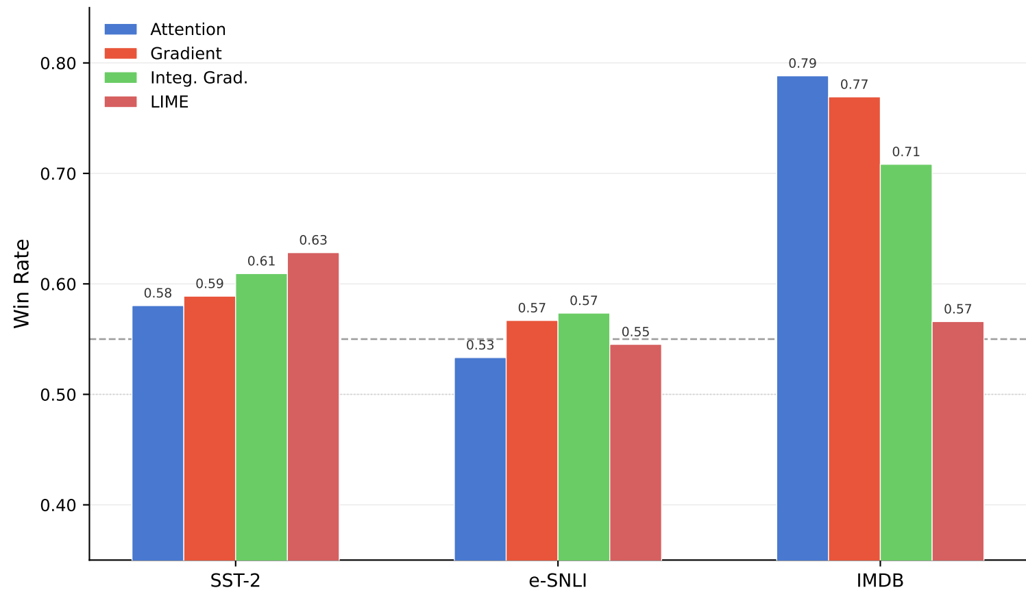
Encoder Model (BERT) Retrieval Win Rates by Extractor
