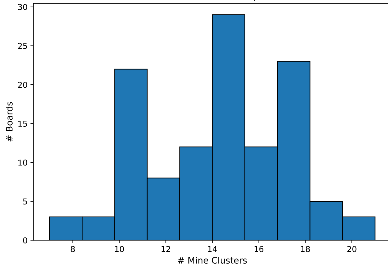
Number of Mine Clusters per Board
