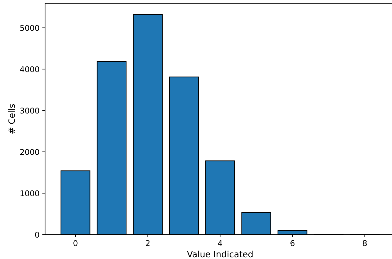
Distribution of Number of Cells with Values
