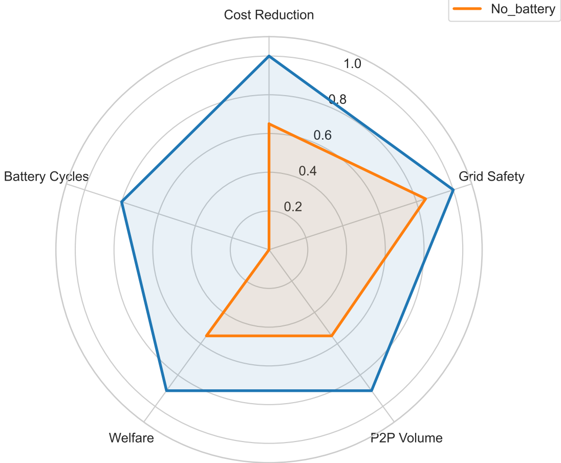
Ablation Study Multi-Metric Performance Radar Summary
