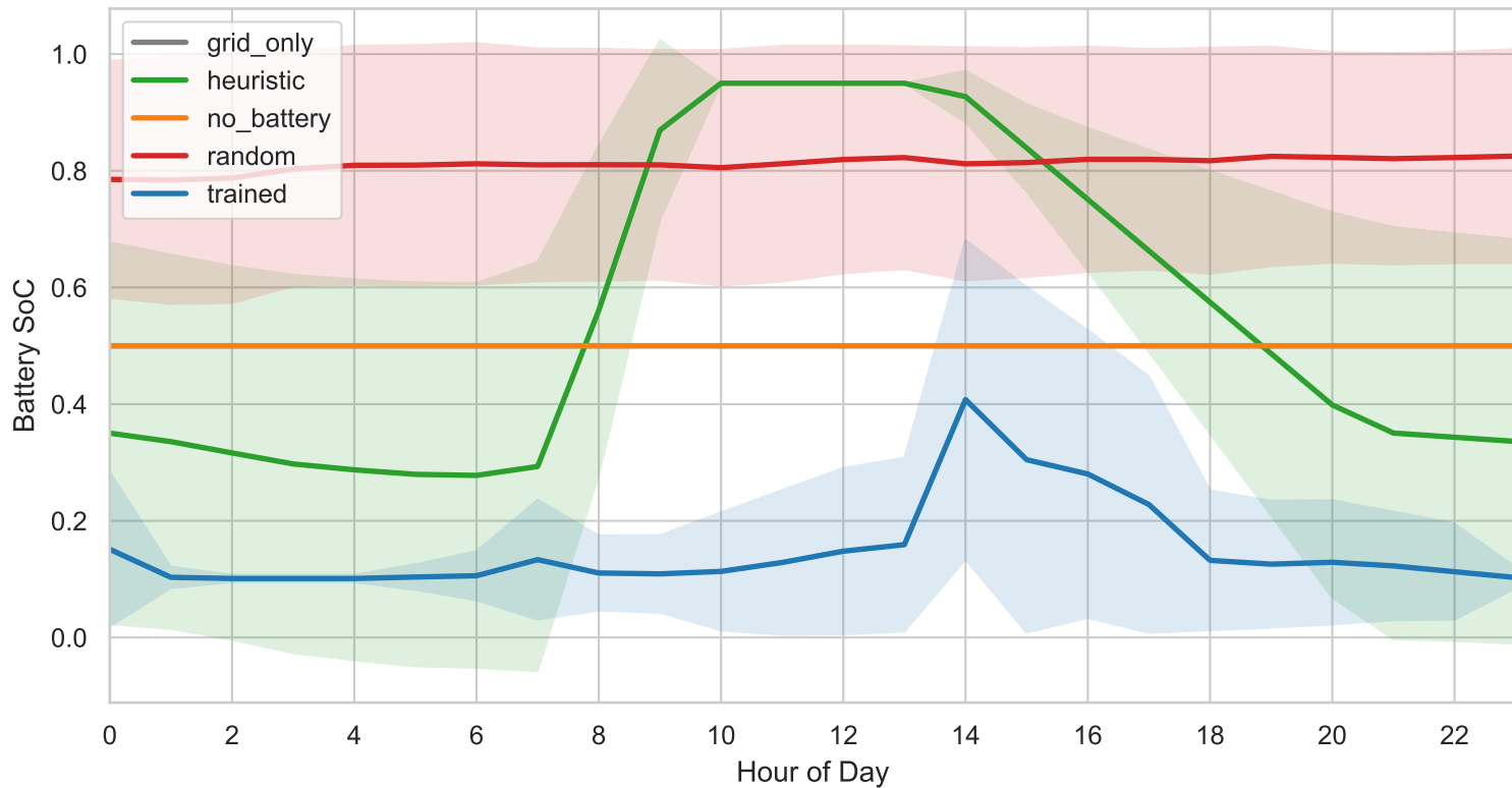
College Battery 24-Hour State-of-Charge (SoC) Profile
