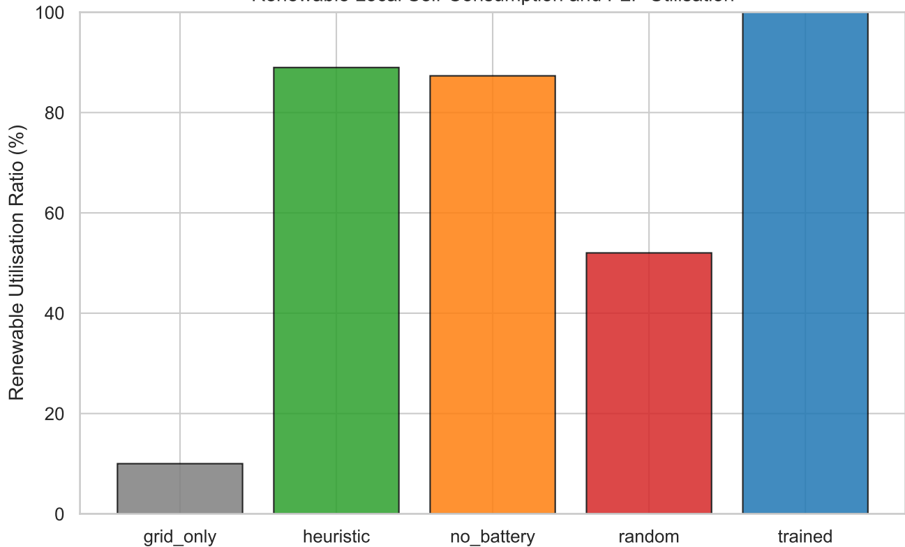
Renewable Local Self-Consumption and P2P Utilisation
