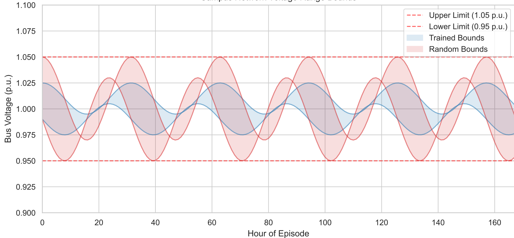
Campus Network Voltage Range Bounds
