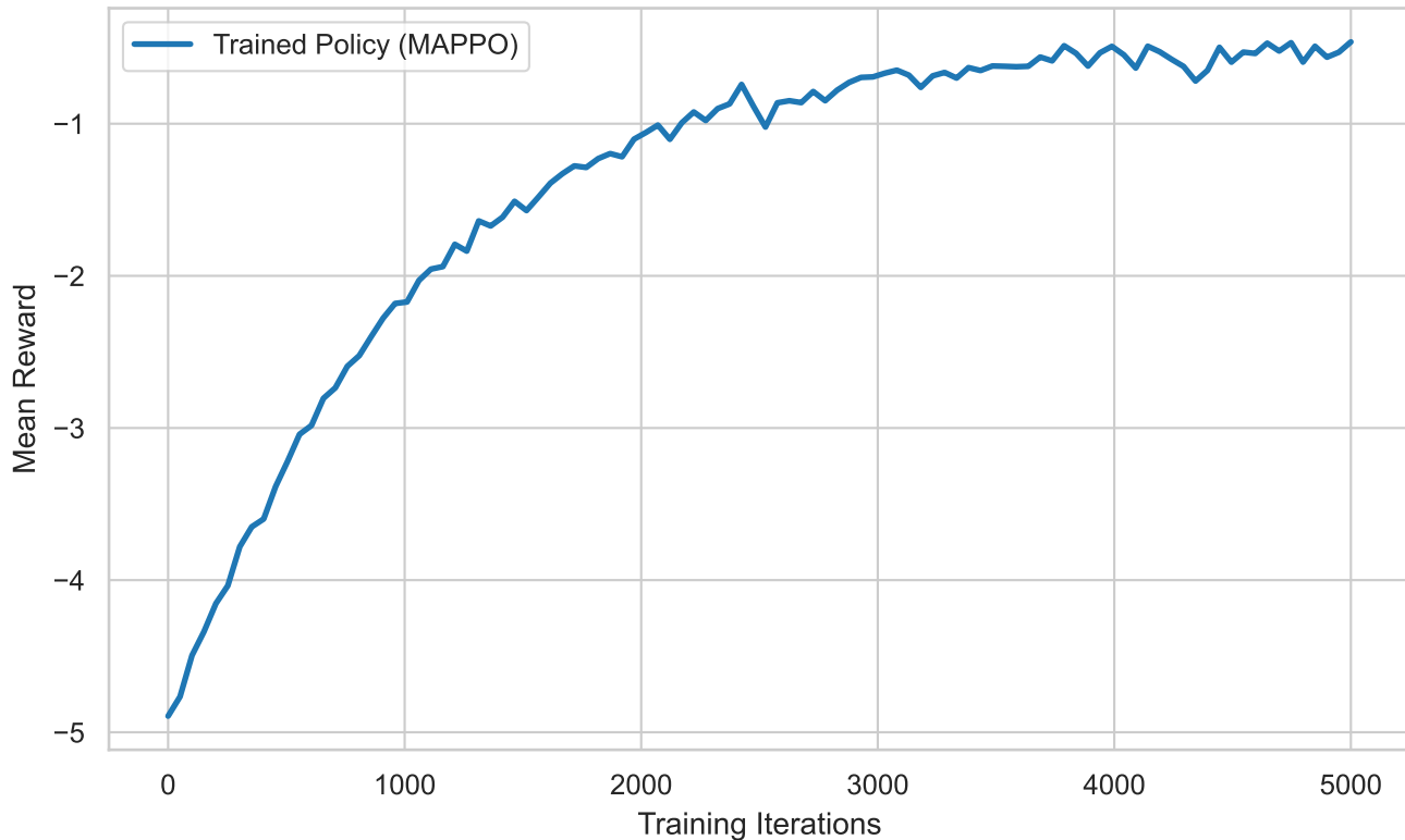
Training Convergence Performance
