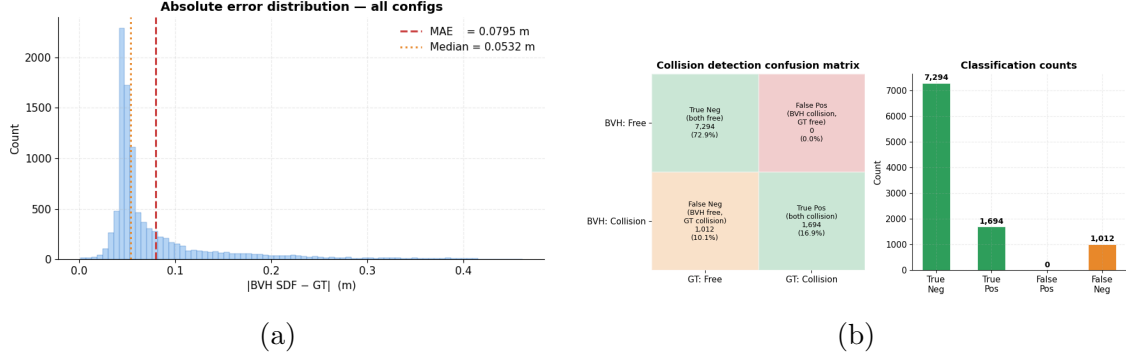
Figure 8: a) Error distribution b) Confusion matrix
