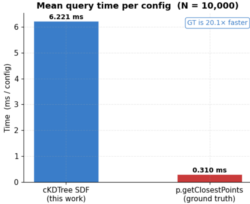
Figure 7: Time taken for sdf computation
