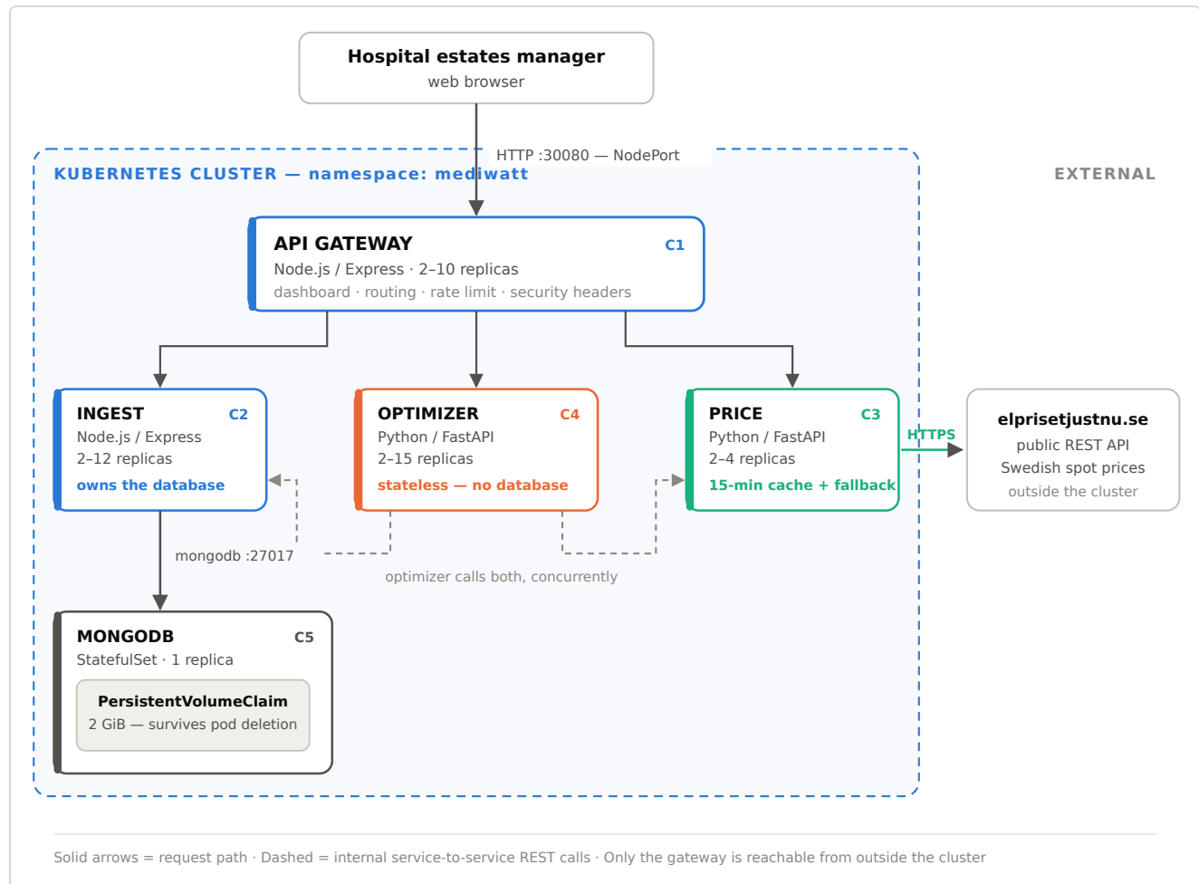
Figure 1 — MediWatt component and deployment architecture. C1–C5 are the logical components mapped in Table 2.1.
