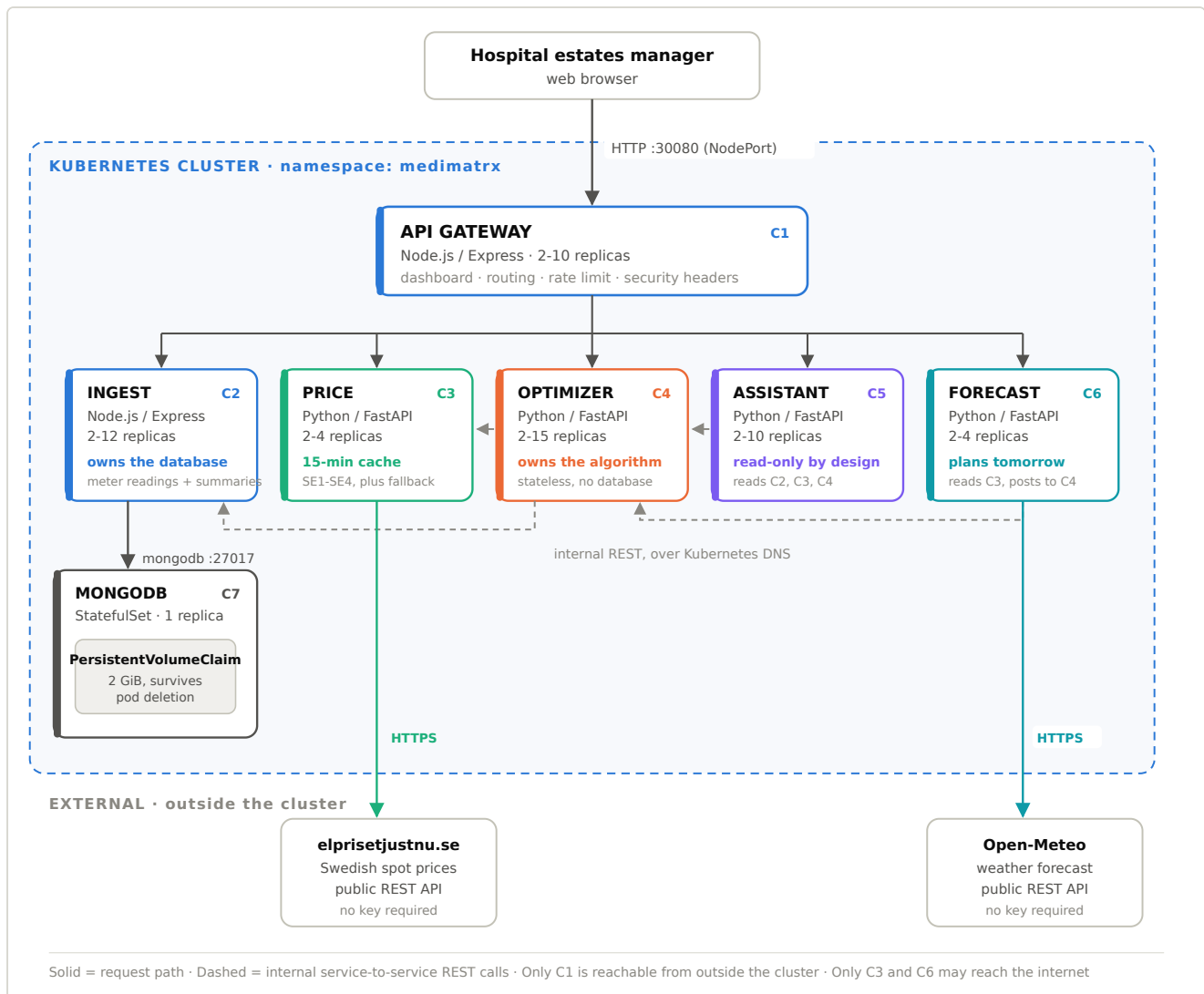
Figure 1: MediMatrix component and deployment architecture. C1 to C7 are the logical components mapped in Table 2.1.
