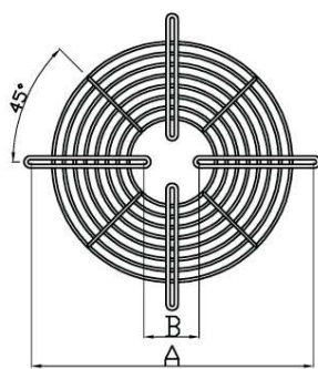
FRONT VIEW W/O FAN
