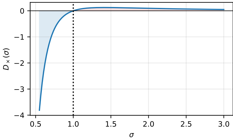
Cross-dissipation sign transition
