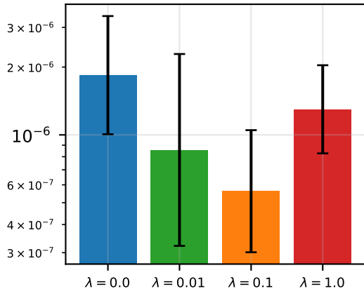
(a) L_{\text{phys}} at convergence
