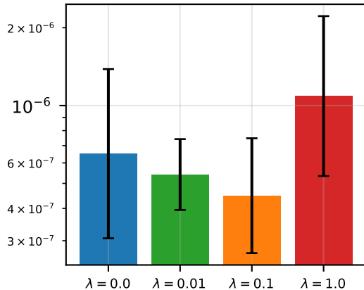
(b) ODE consistency (off-grid)
