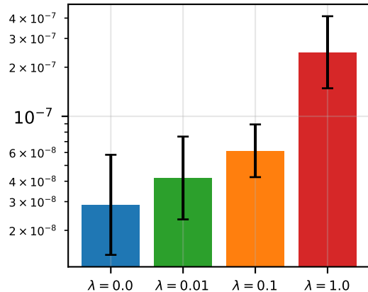
(c) E_{\text{traj}} (test)
