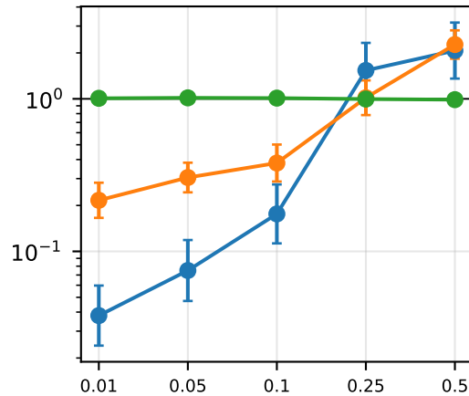
(A) PDE target, reduced-ODE baseline
