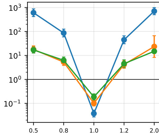
(C) Fisher, misspecified \kappa
