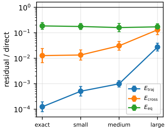
(A) PDE target, reduced-ODE baseline
