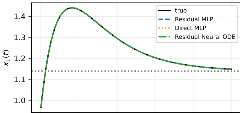
Non-normal transfer system ( c = 0.97 , \gamma = 0.28 )
