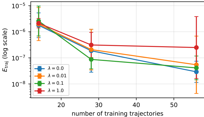
Data efficiency
