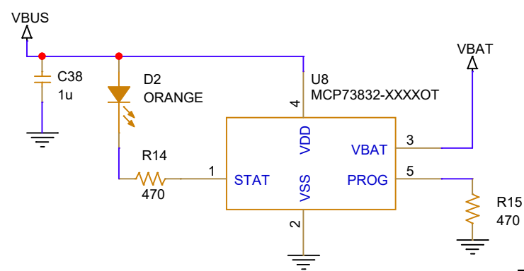
Battery Charging
