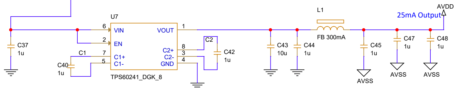
5V Step Up
