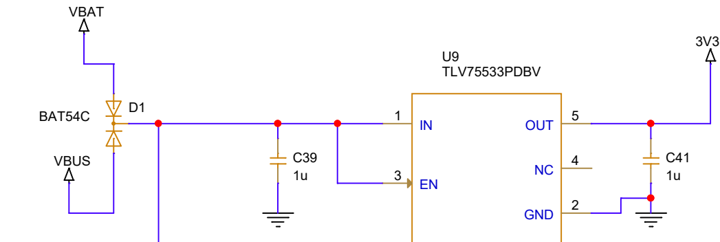
3.3V Linear Regulator
