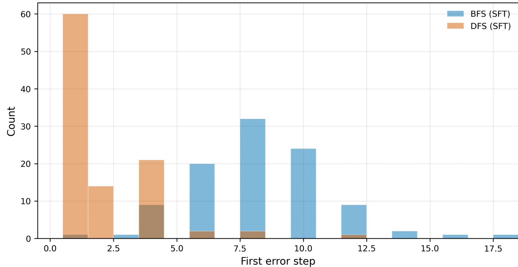
First-error step distribution
