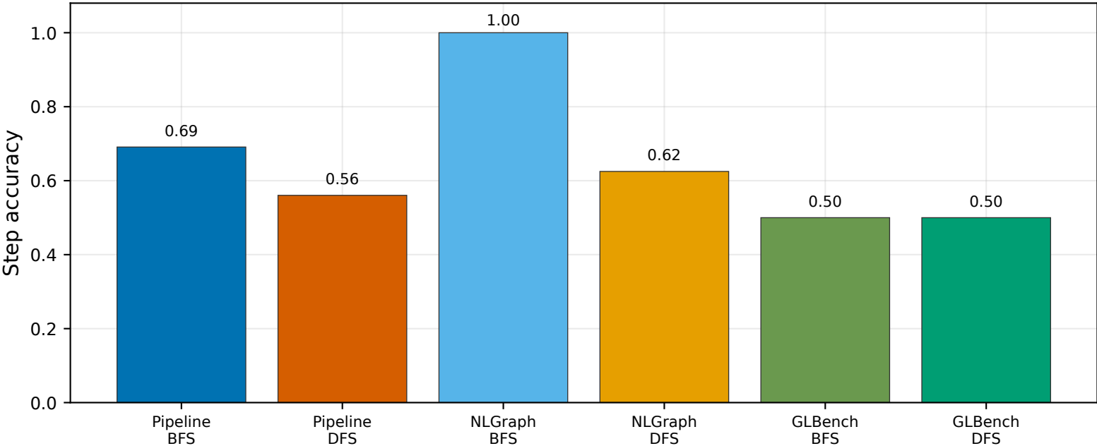
Qwen2.5-7B-Instruct: pipeline / NLGraph = pre-DAGger SFT; GLBench = BFS SFT+DAGger R1 on glbench_eval_quick2x (2 BFS + 2 DFS rows, teacher-forced)
