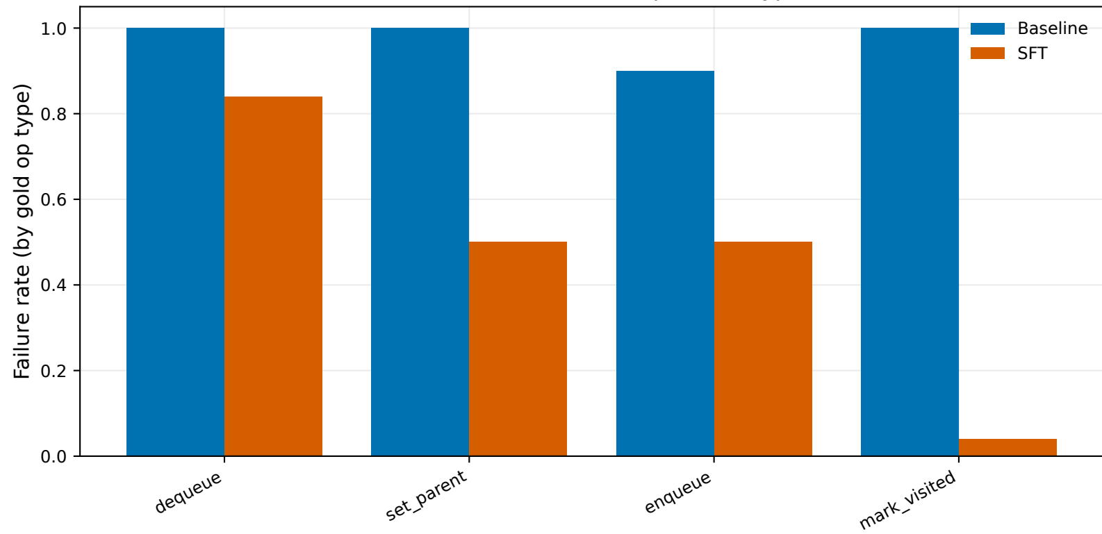
Where the model fails: operation type
