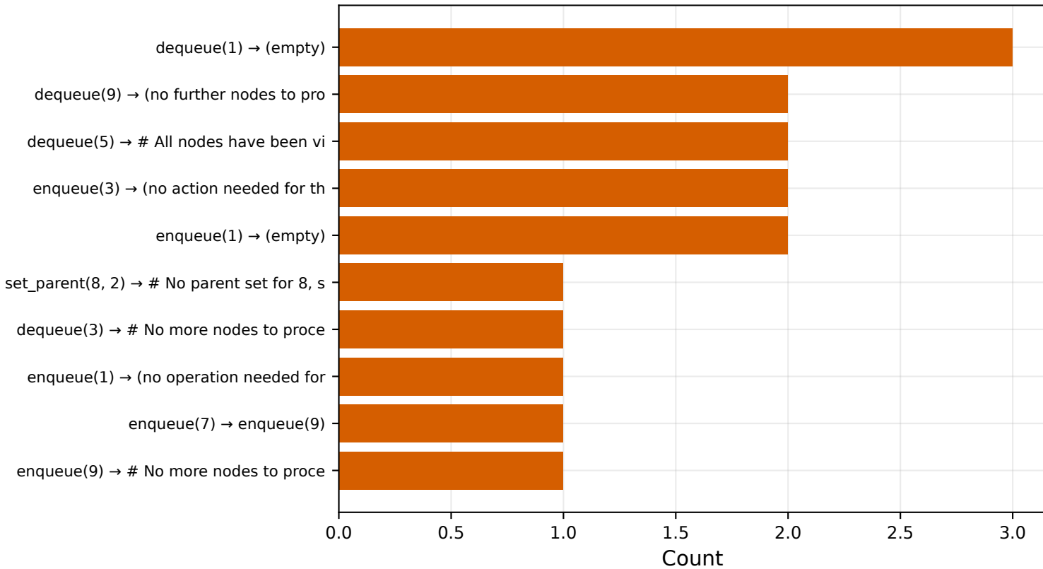
Top gold→predicted confusions (SFT)
