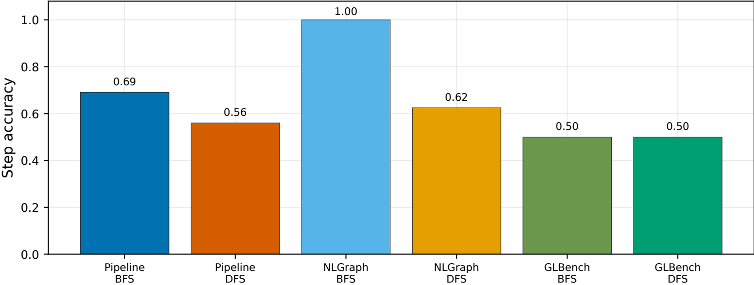
Green bars (positions 5-6): GLBench step accuracy. Bars 1-4: pipeline / NLGraph.
