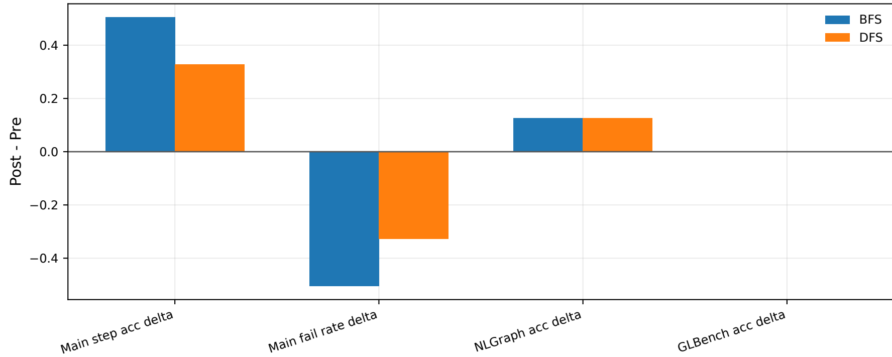
DAGger gain/loss deltas by algorithm
