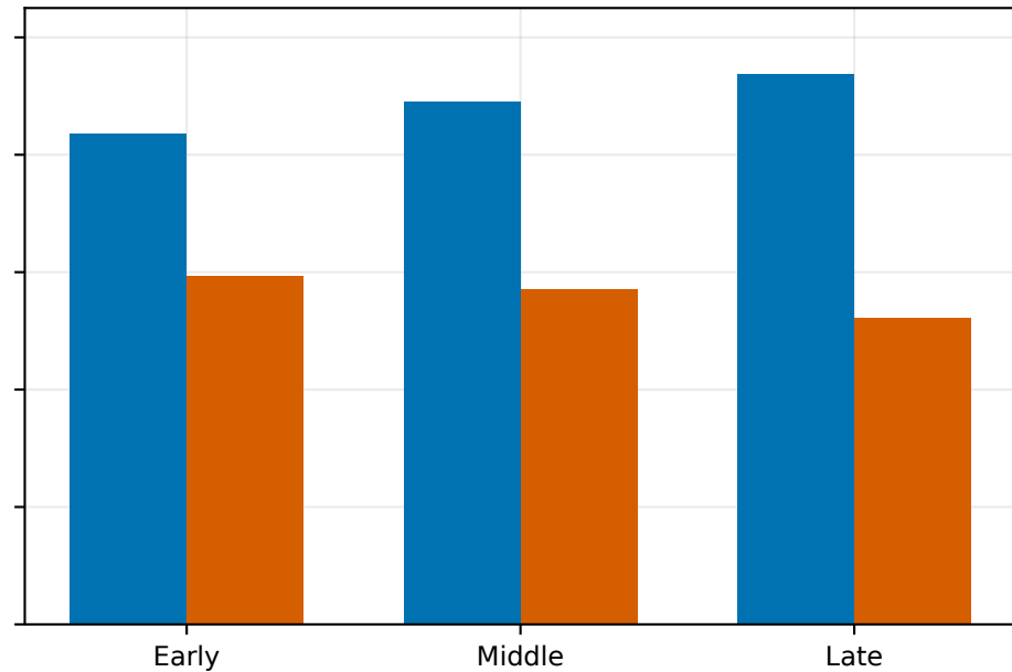
DFS
